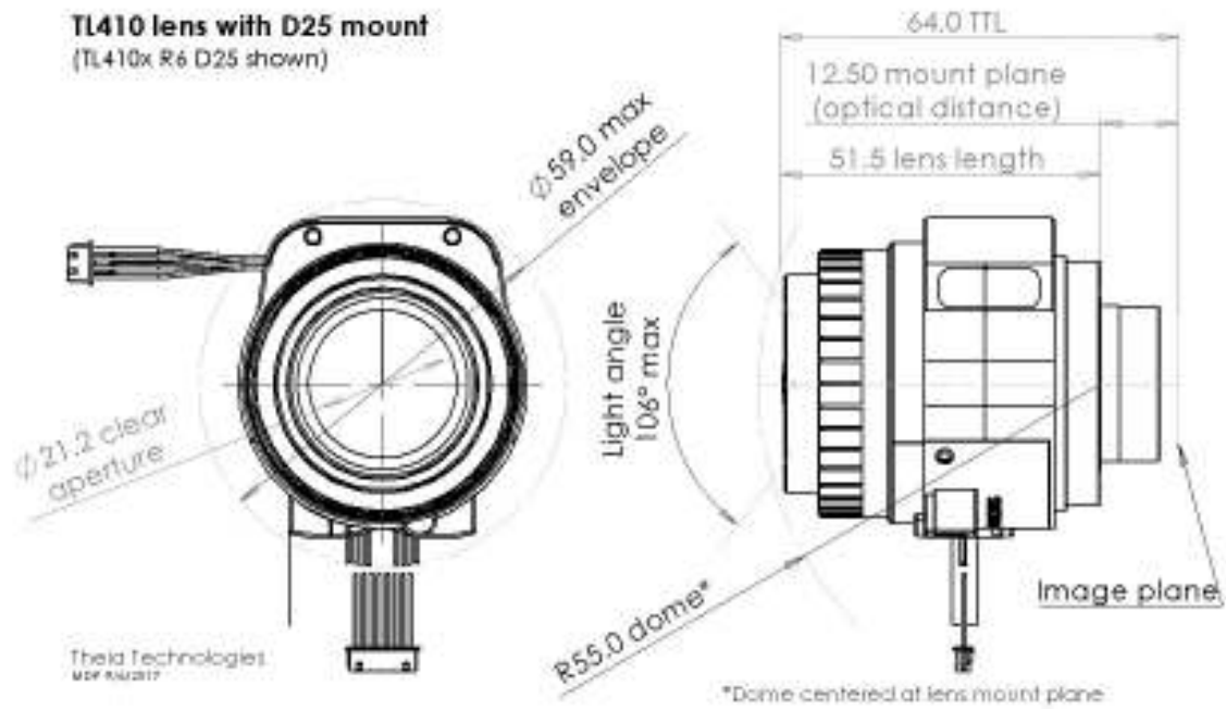
SL410 lens
