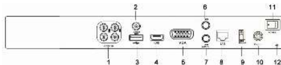
Figure 1.6 Rear Panel of DS-7204HVI/HFI/HWI-SH, DS-7204HVI-SV and DS-7204HWI-SV
