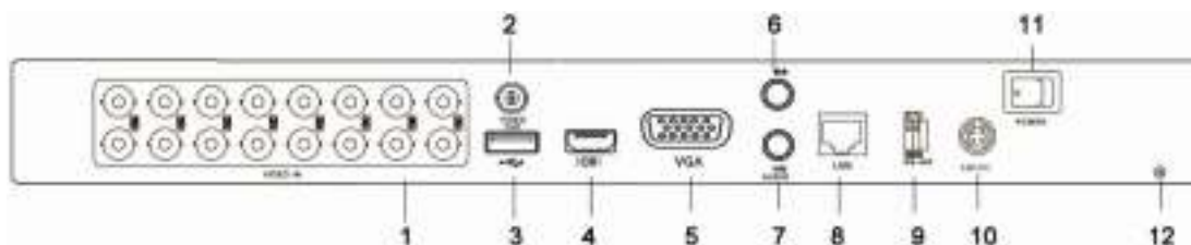
Figure 1.8 Rear Panel of DS-7216HFI-SH and DS-7216HWI-SH
