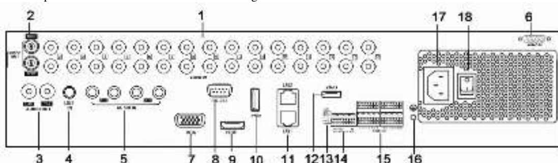
Figure 1.12 Rear Panel of DS-8132HCL-SH, DS-8132HFSI-SH and DS-8132HWSI-SH
