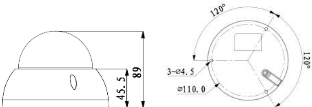
Figure 1-2 Dimension illustration
