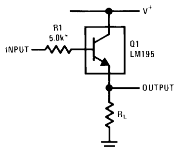
Figure 33. Emitter Follower
